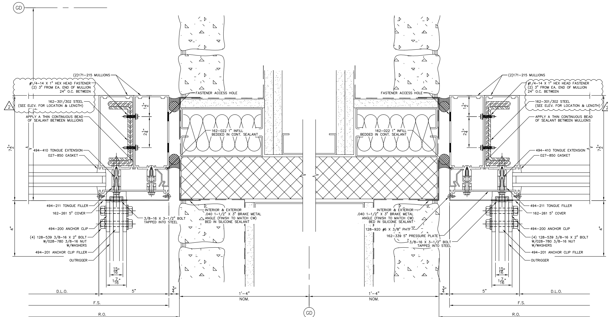
1 CURTAIN WALL JAMB W/SUNSHADE AT FIN WALL 3 A4.11 SCALE 5 A4.11
