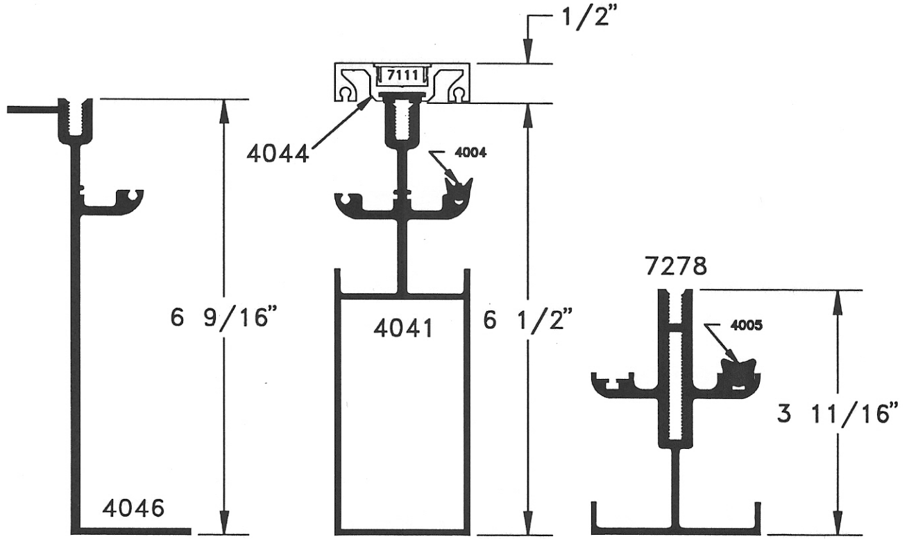
GUTTER
