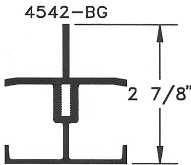
PURLIN
